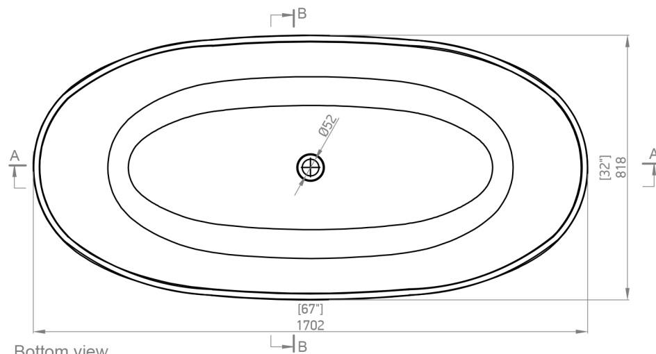
Bottom view
